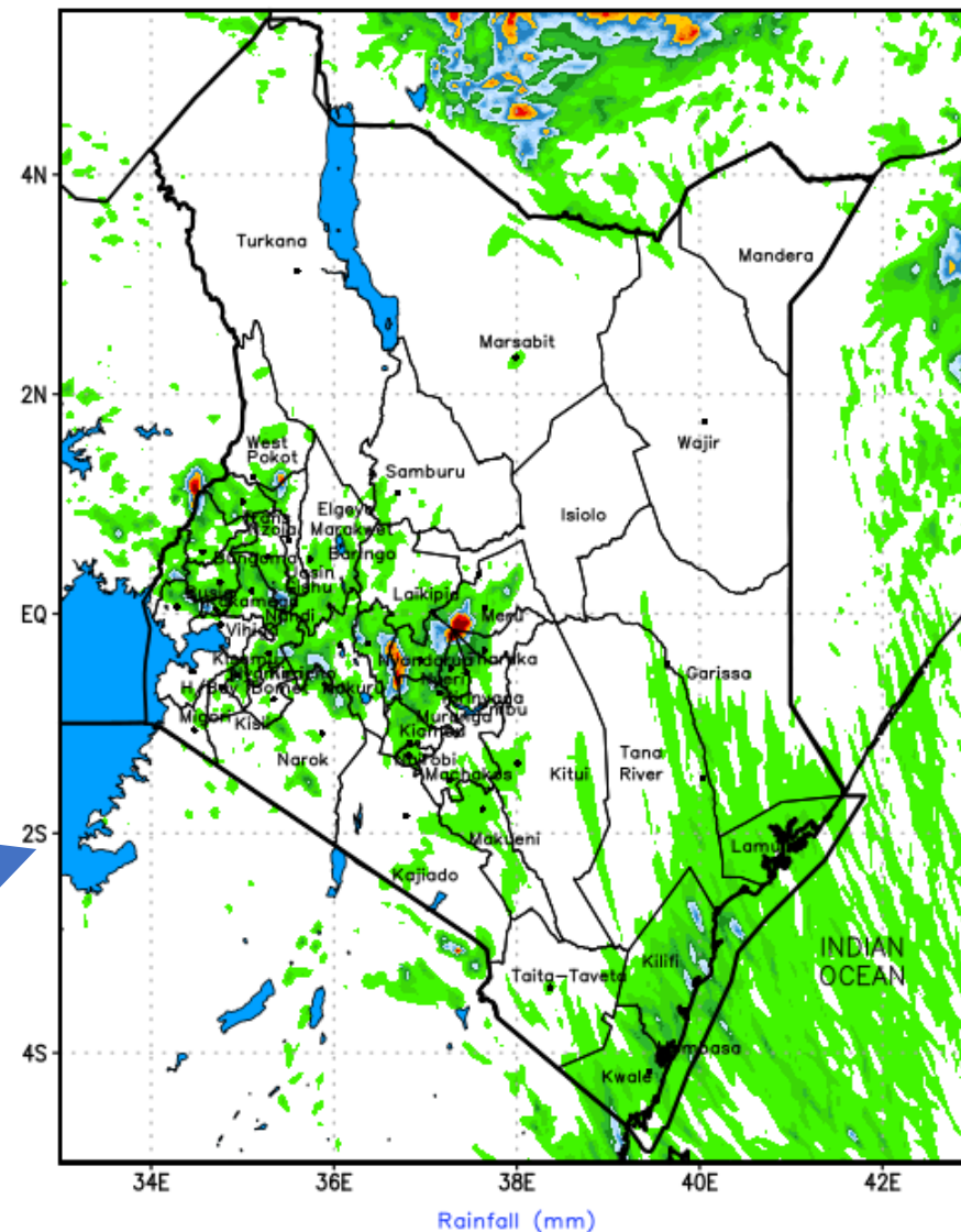
WEEKLY CUMULATIVE RAINFALL FORECAST Valid 0600Hrs 14OCT to 0600Hrs 20OCT 2025
