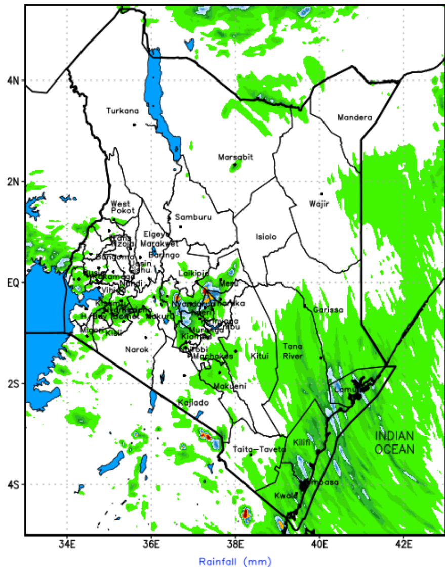
WEEKLY CUMULATIVE RAINFALL FORECAST Valid 0600Hrs 07OCT to 0600Hrs 14OCT 2025
